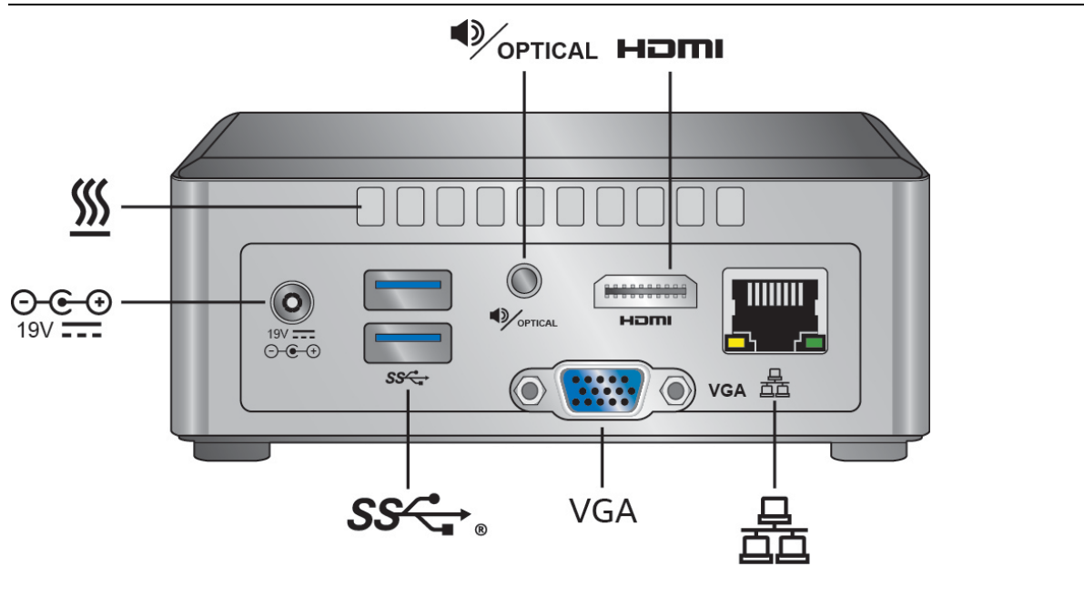
Figure 21. Intel NUC Kit NUC6CAYH/NUC6CAYS Features – Rear
